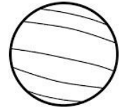
Neptune
